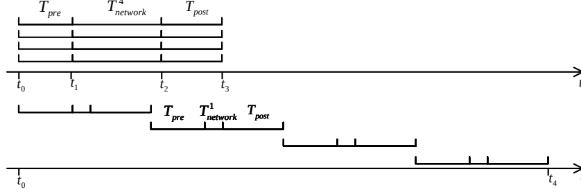
Figure 3: An example of sequential and parallel migrations
