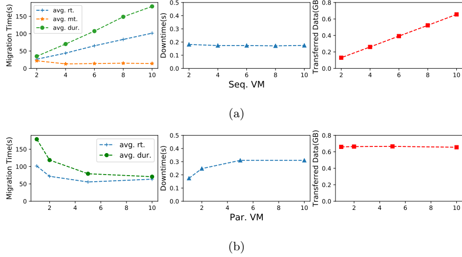
Figure 7: (a) Sequential migrations with different number of VMs; and (b) Multiple live migrations of 10 VMs where x-axis indicates the max allowed concurrent migration.
