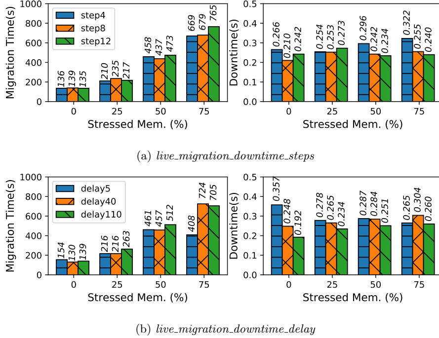
Figure 6: Live migrations based on different step and delay settings
